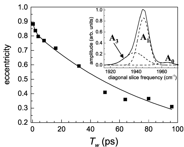
Fig. 4 Eccentricity of the A_1 substate of MbCO. The line through the data is a bi-exponential fit. Inset: Normalized diagonal slice through the 2D IR data for MbCO at T_w = 0.5 ps. The spectrum is fit to three Gaussian curves, centered at frequencies of the A_i bands in MbCO.
